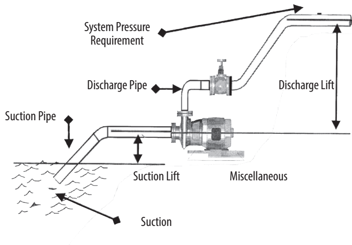
Figure 9-1: Determining Total Dynamic Head (TDH) IA Certified Irrigation Contractor Workbook. Chapter 9 Part No. AXIA-CICW $49.00
